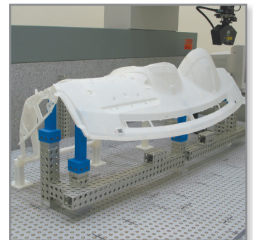
Image 3: The CMM scan showed the ABS Prototype was within tolerance.
