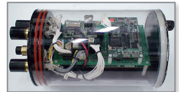
Image 2: Electronics enclosure prototyped with FDM.
